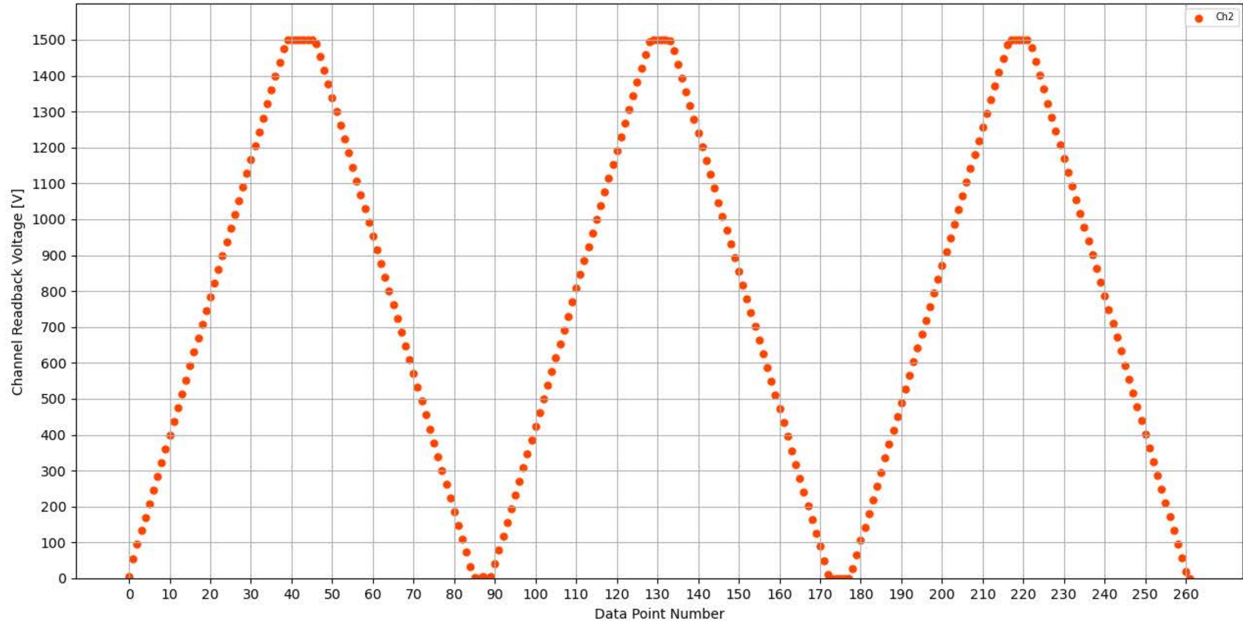
Voltage Ramp Test (Python) Bd #309, Slot #9, Ch #2
