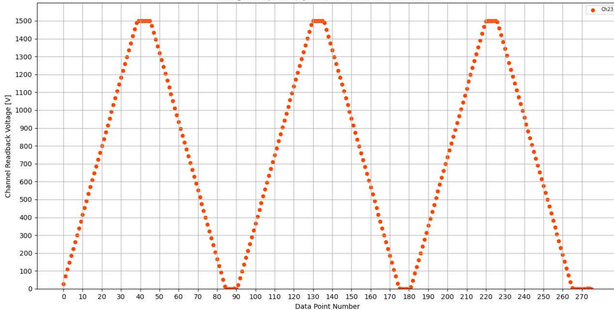
Voltage Ramp Test (Python) Bd #309, Slot #9, Ch #23
