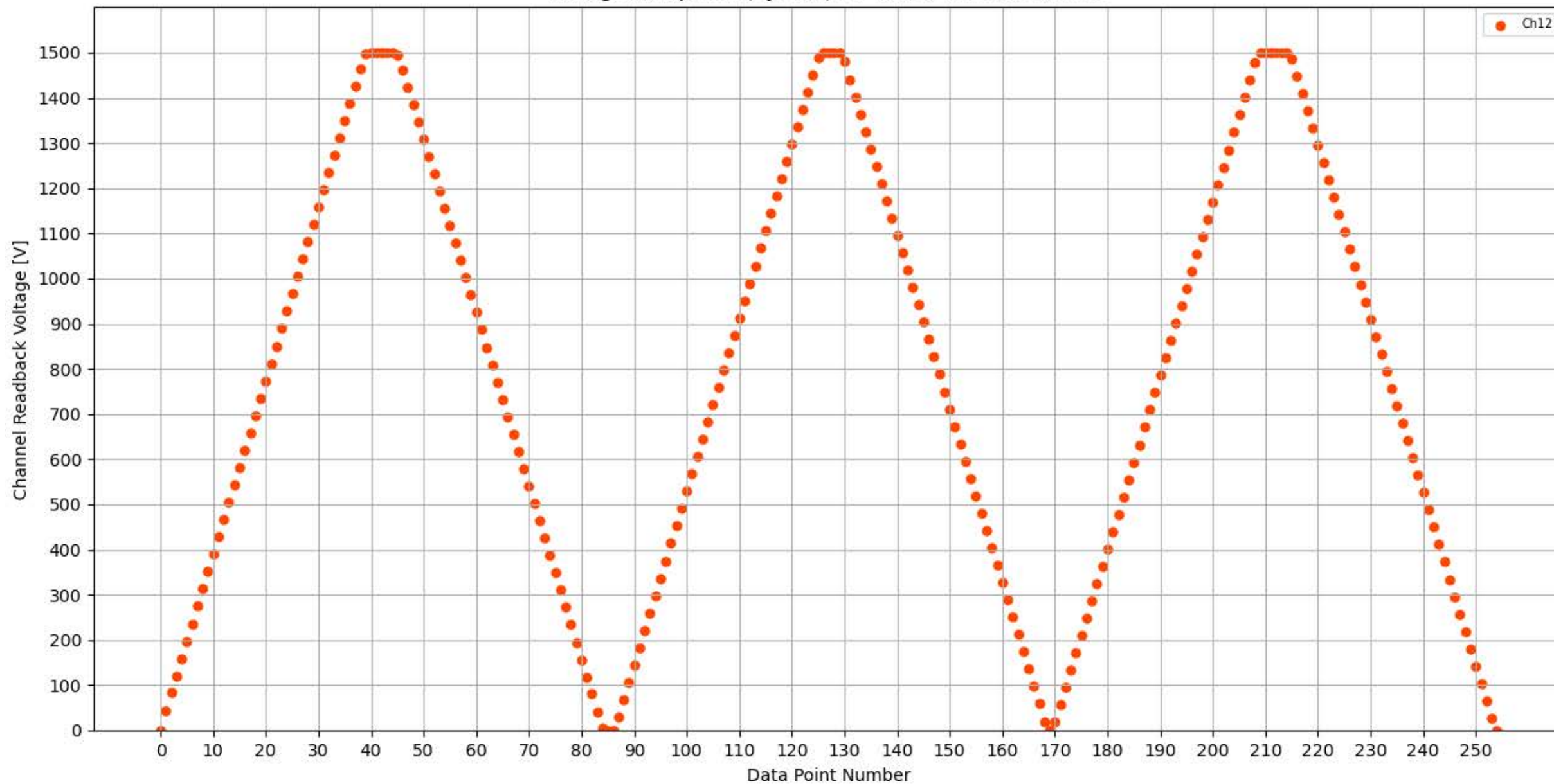
Voltage Ramp Test (Python) Bd #309, Slot #9, Ch #12
