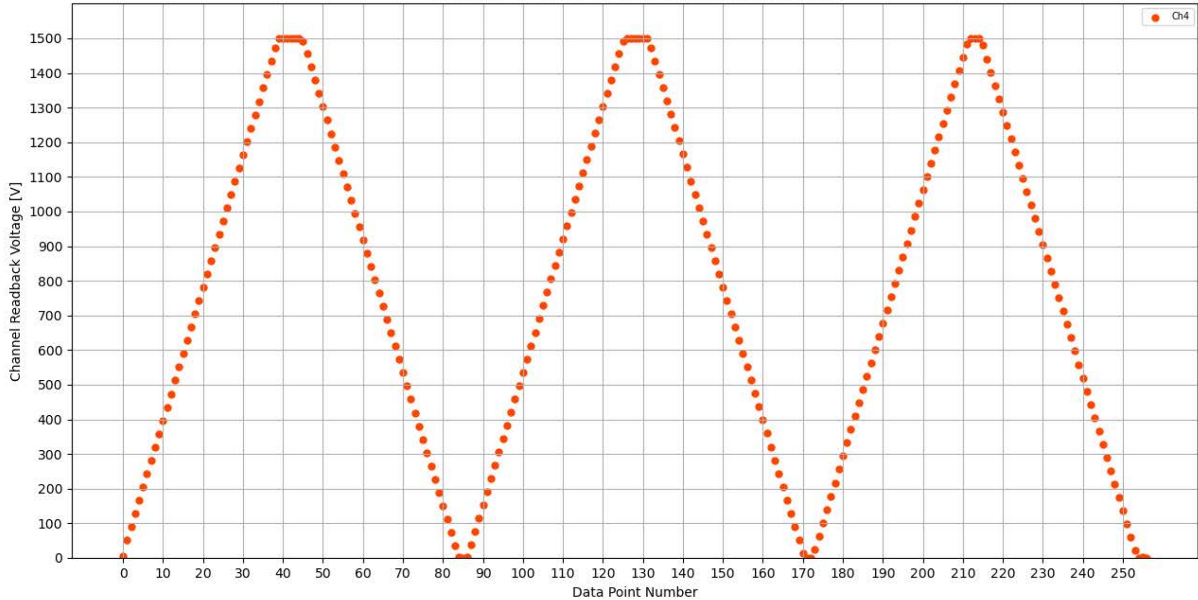
Voltage Ramp Test (Python) Bd #309, Slot #9, Ch #4
