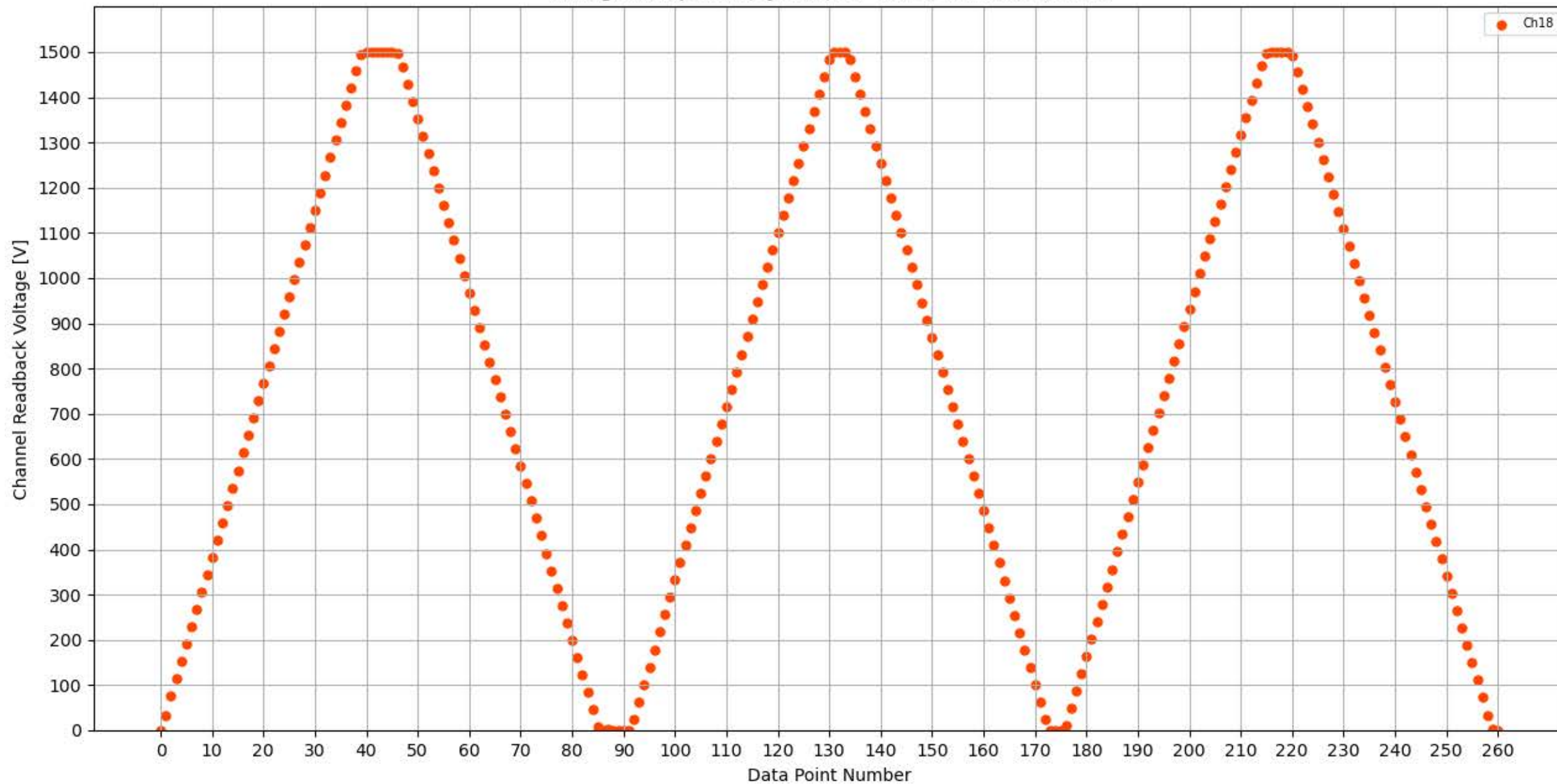
Voltage Ramp Test (Python) Bd #309, Slot #9, Ch #18
