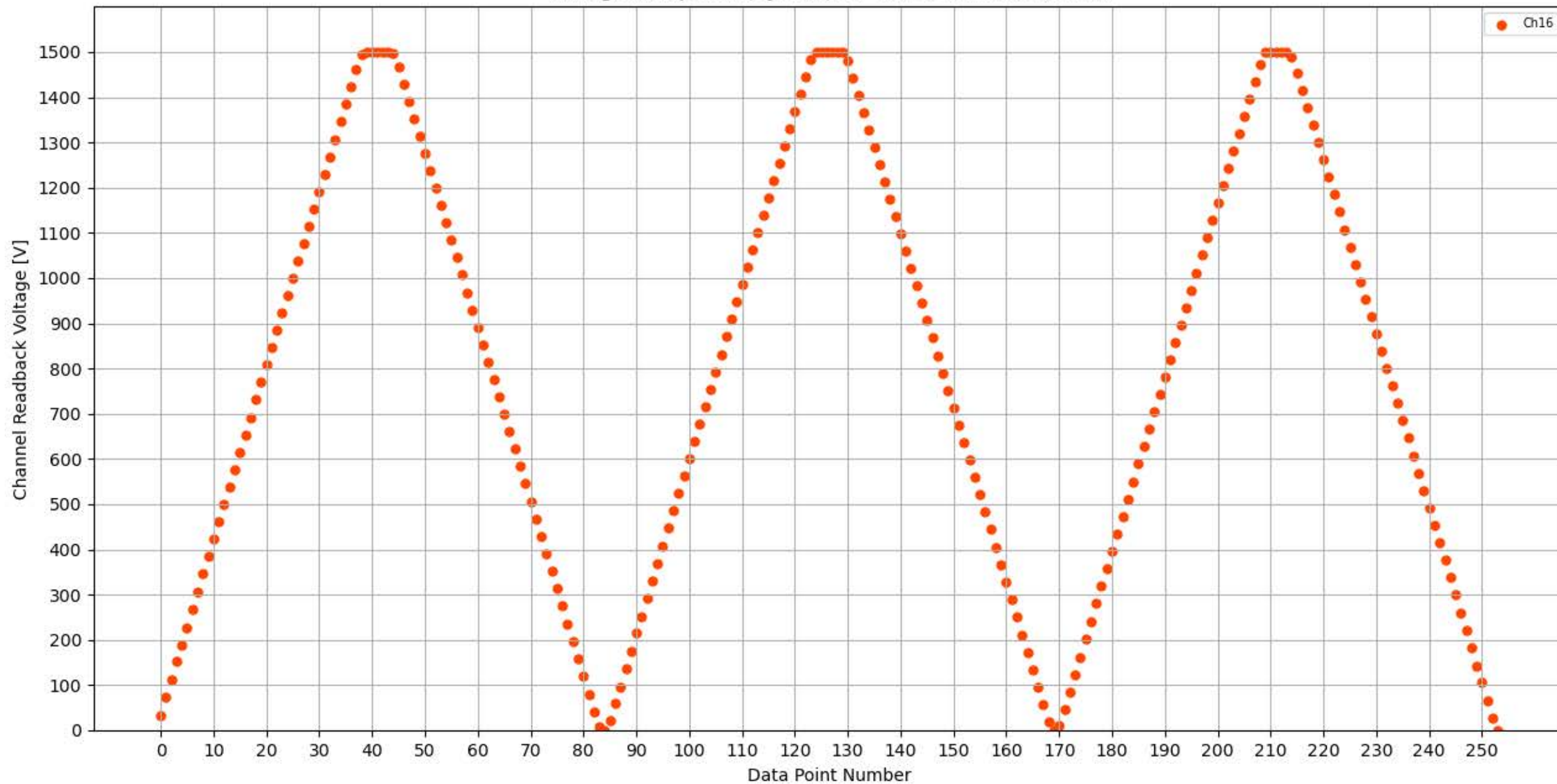
Voltage Ramp Test (Python) Bd #309, Slot #9, Ch #16
