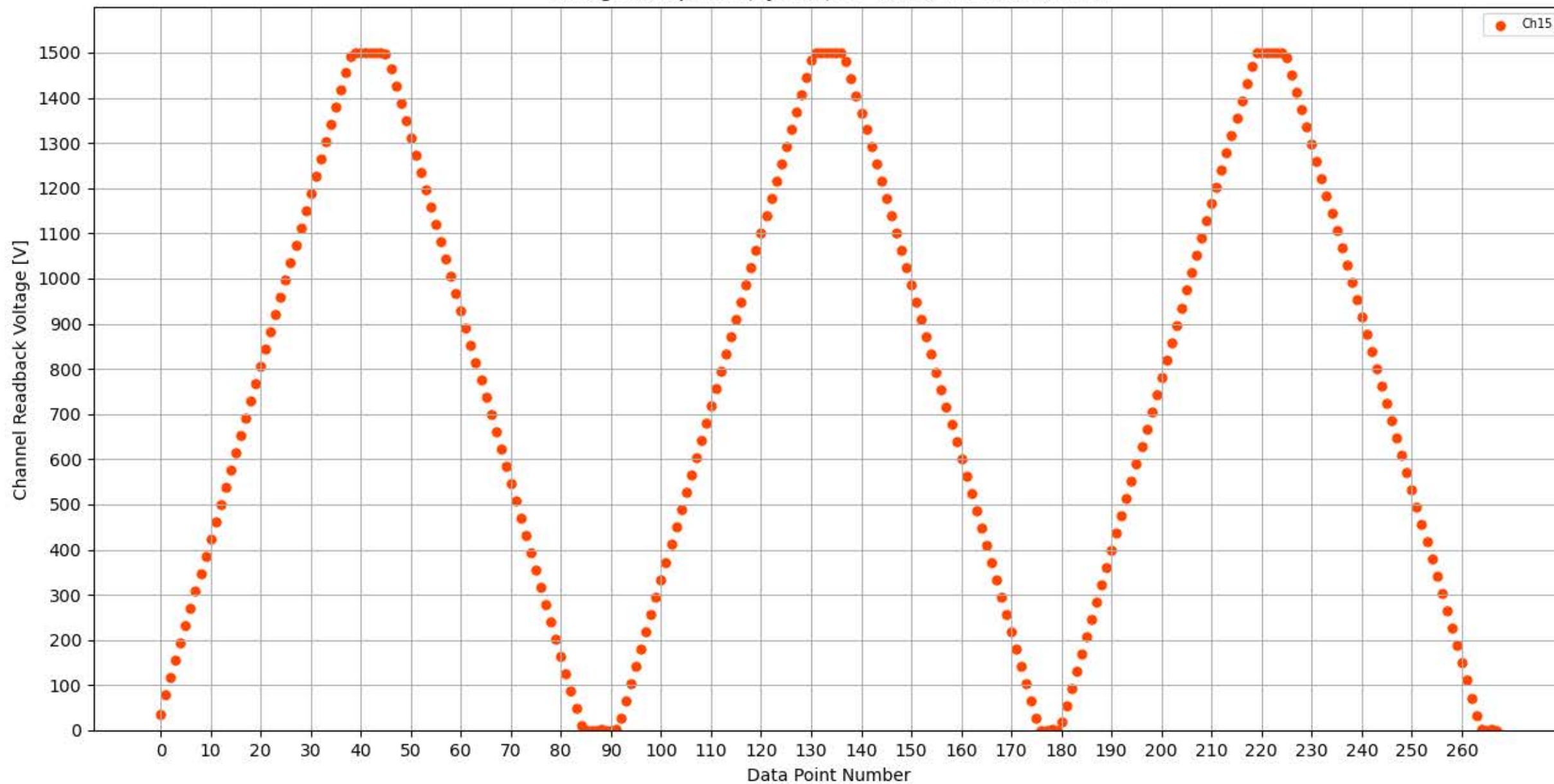
Voltage Ramp Test (Python) Bd #309, Slot #9, Ch #15
