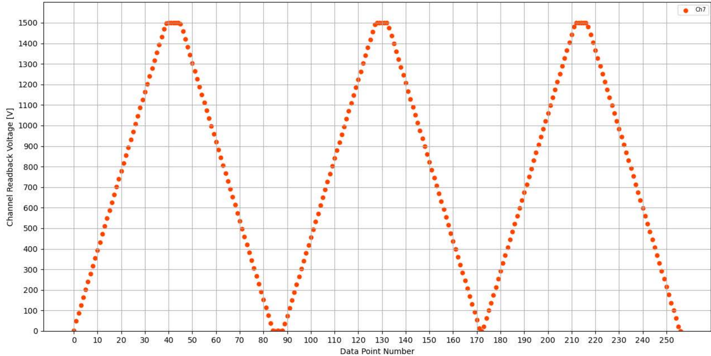
Voltage Ramp Test (Python) Bd #309, Slot #9, Ch #7
