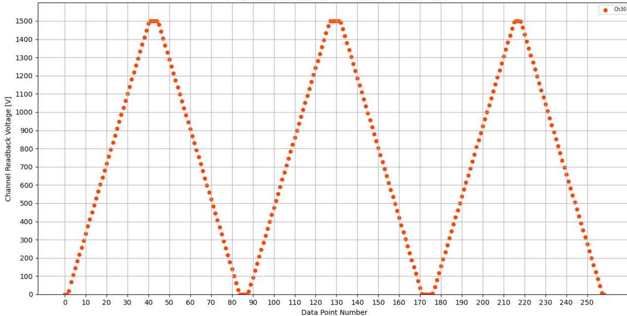
Voltage Ramp Test (Python) Bd #309, Slot #9, Ch #30
