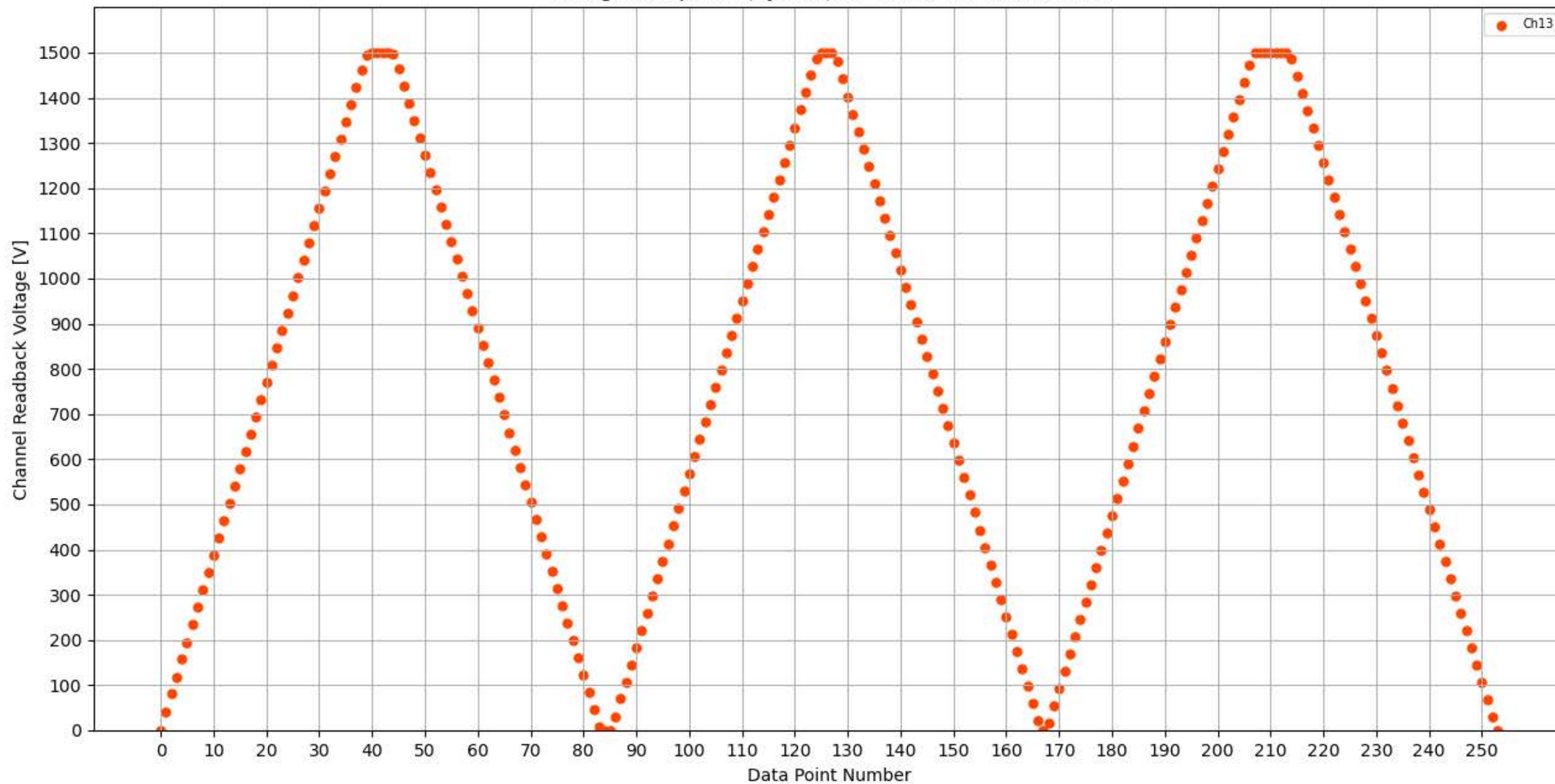
Voltage Ramp Test (Python) Bd #309, Slot #9, Ch #13
