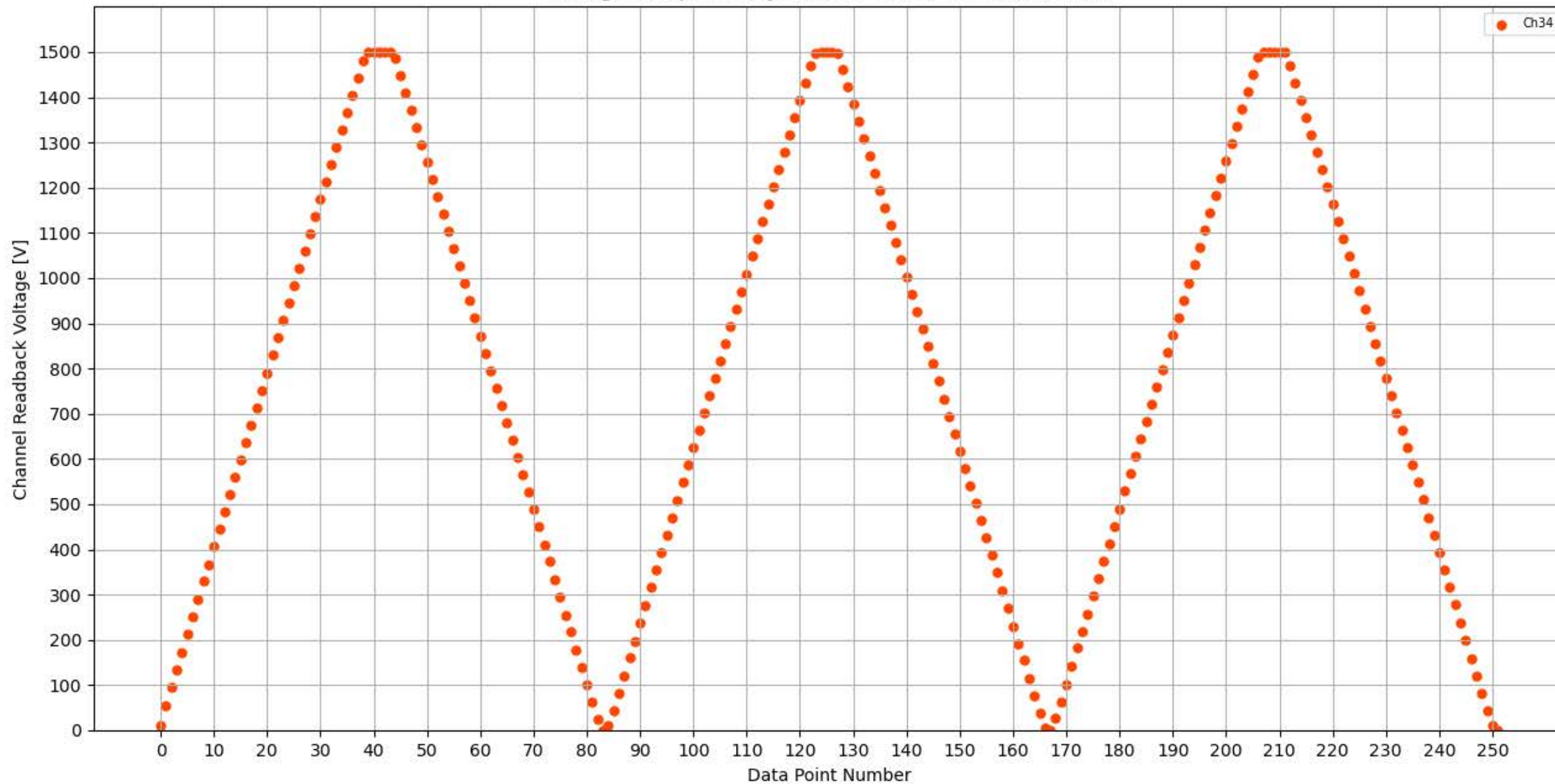
Voltage Ramp Test (Python) Bd #309, Slot #9, Ch #34
