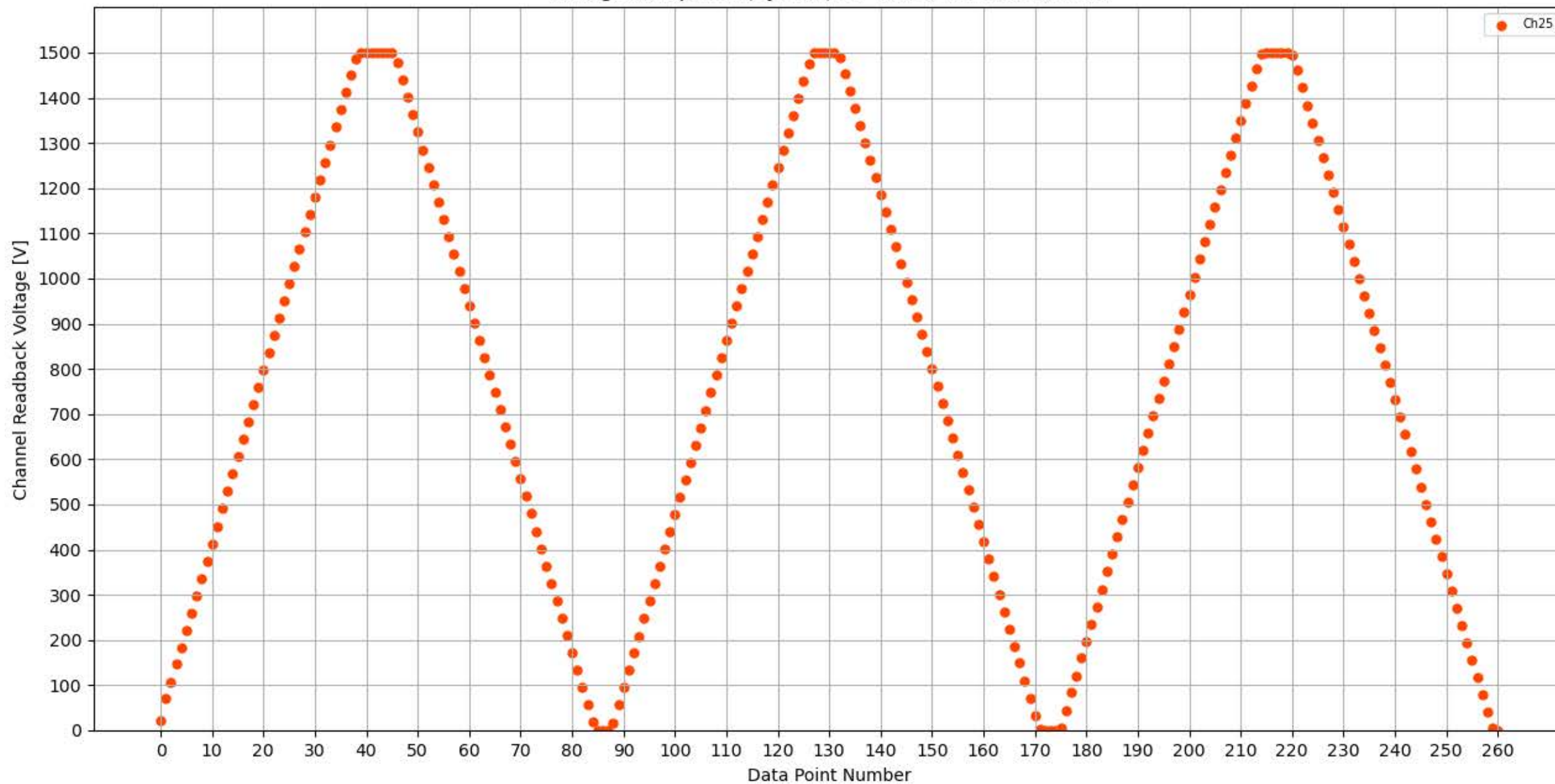
Voltage Ramp Test (Python) Bd #309, Slot #9, Ch #25
