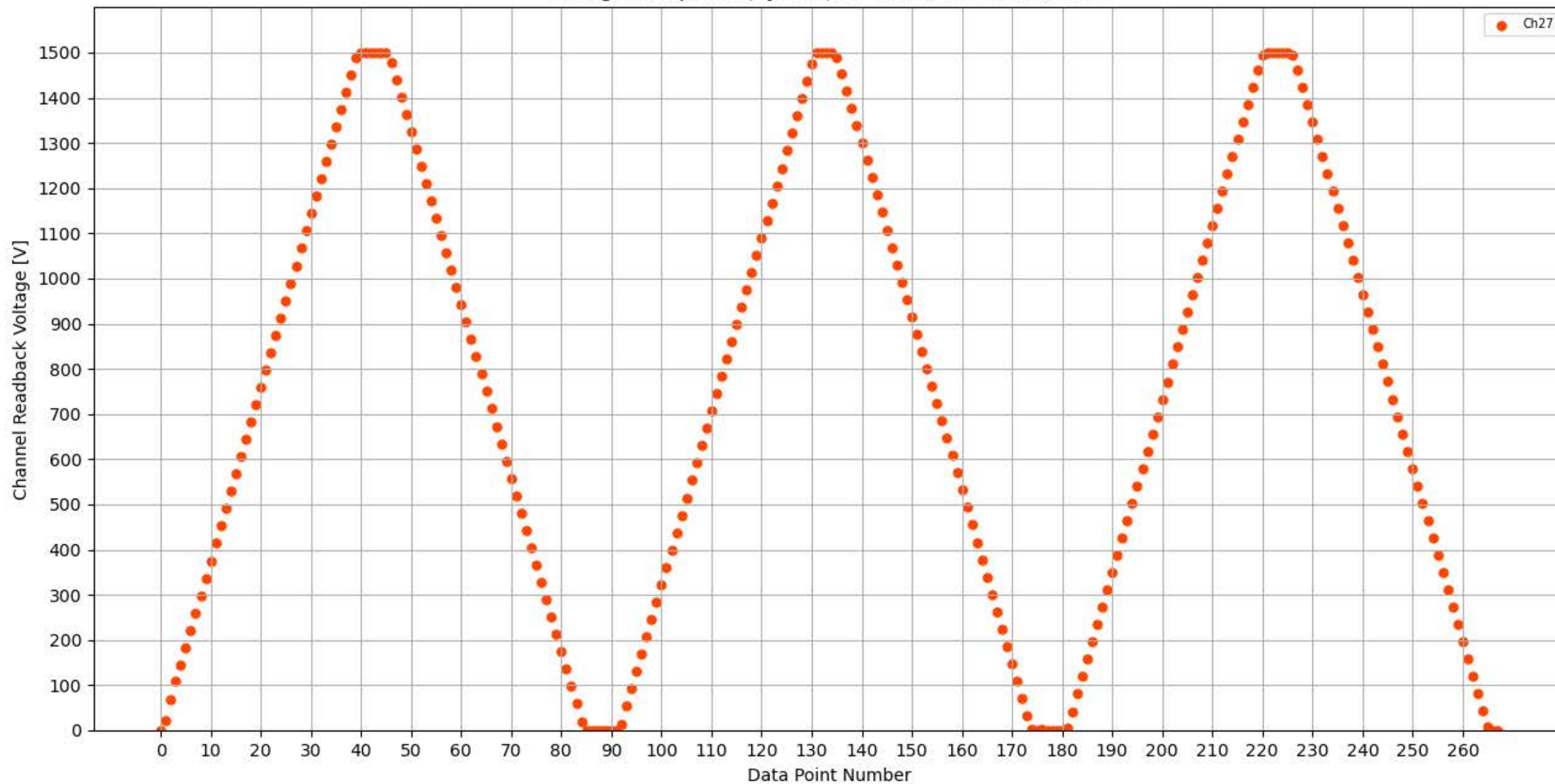
Voltage Ramp Test (Python) Bd #309, Slot #9, Ch #27
