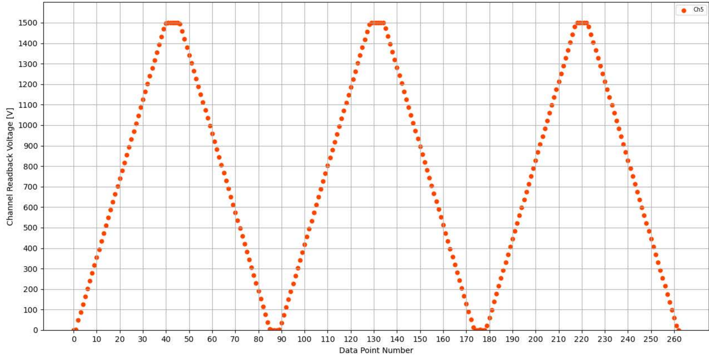
Voltage Ramp Test (Python) Bd #309, Slot #9, Ch #5
