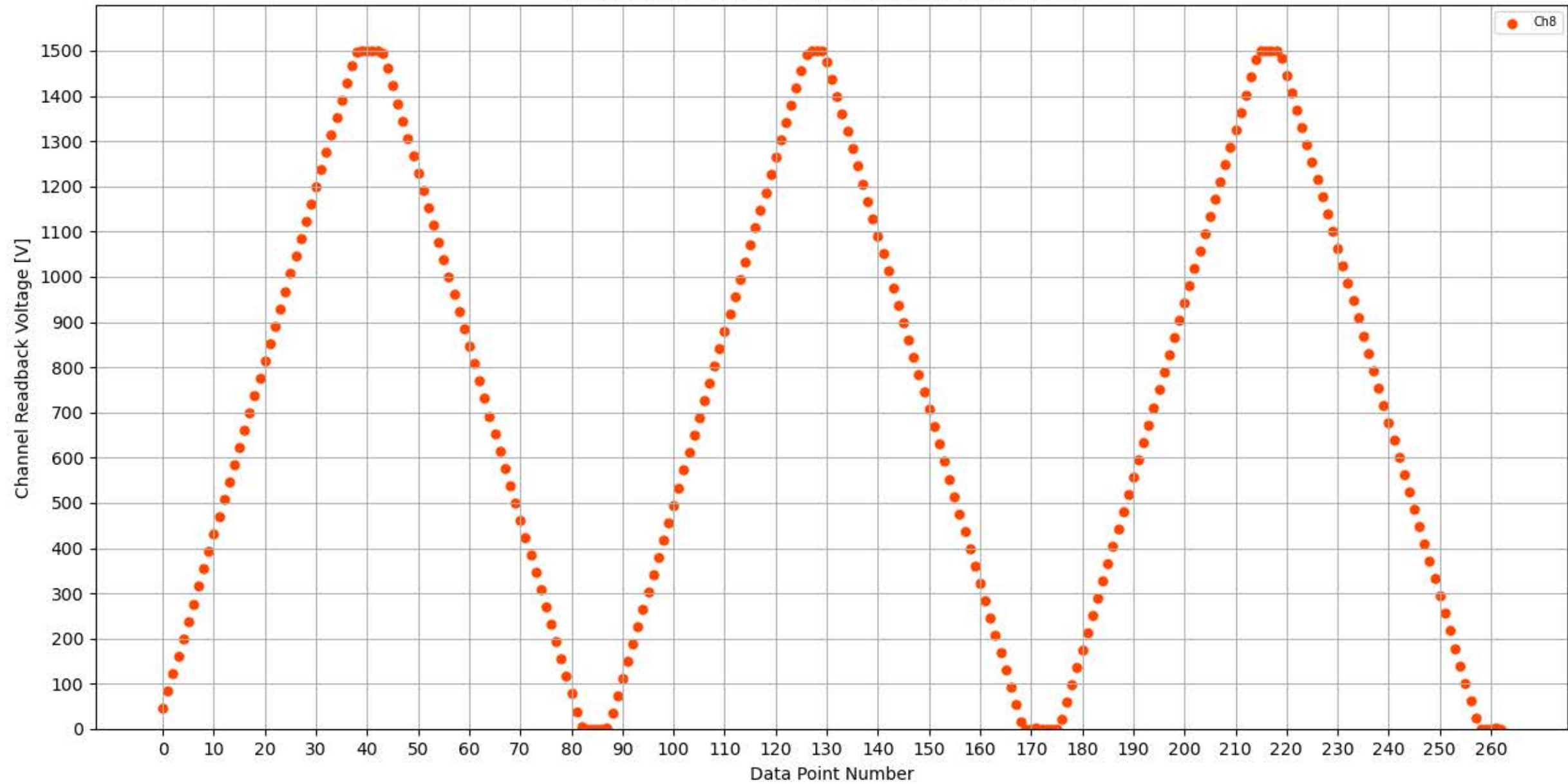
Voltage Ramp Test (Python) Bd #309, Slot #9, Ch #8
