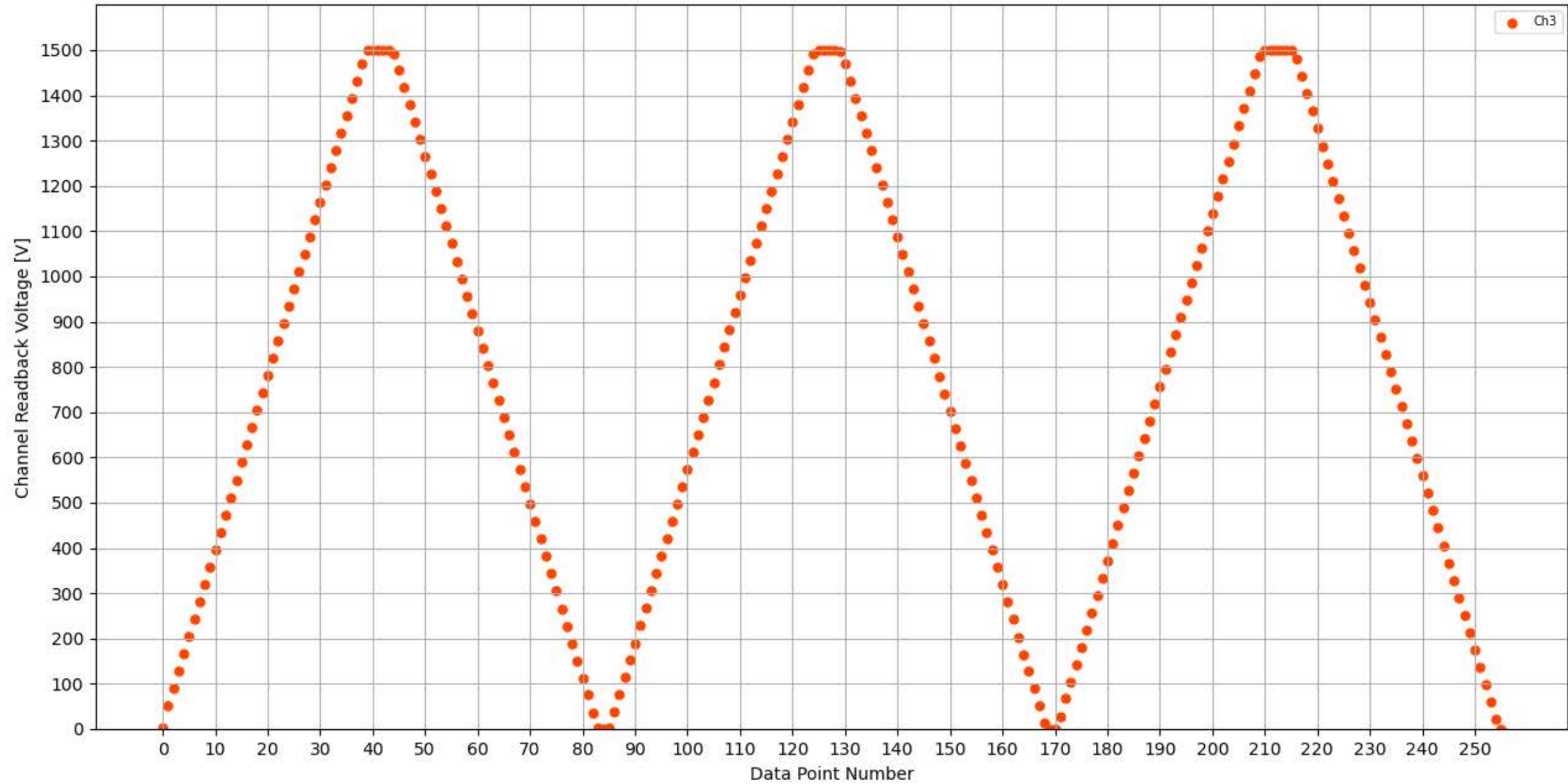
Voltage Ramp Test (Python) Bd #309, Slot #9, Ch #3
