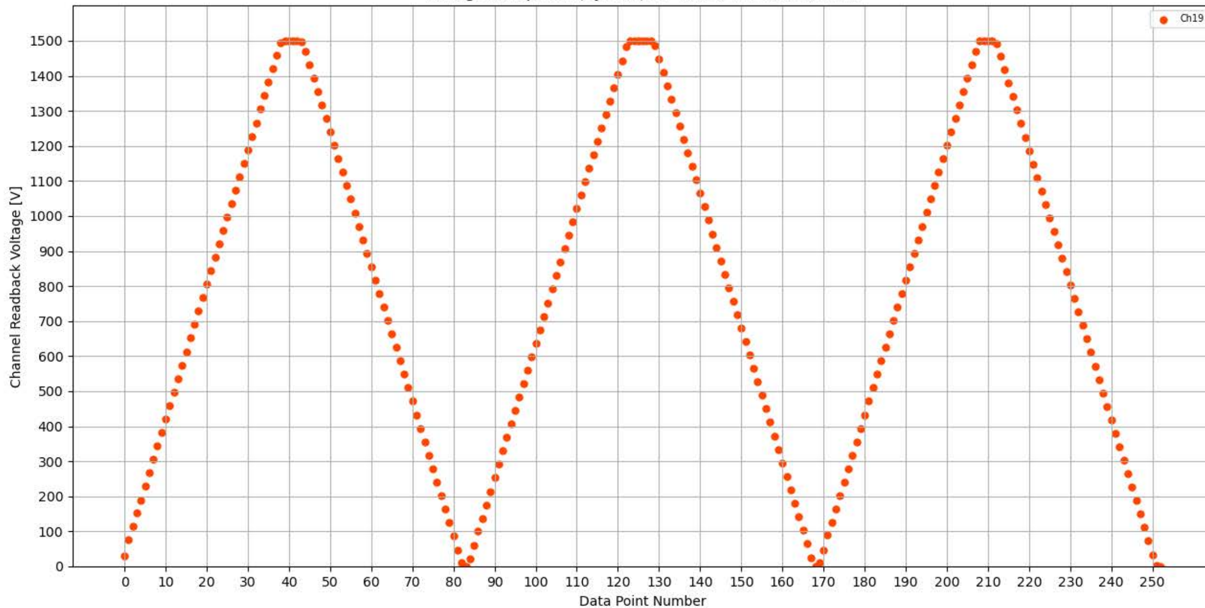
Voltage Ramp Test (Python) Bd #309, Slot #9, Ch #19
