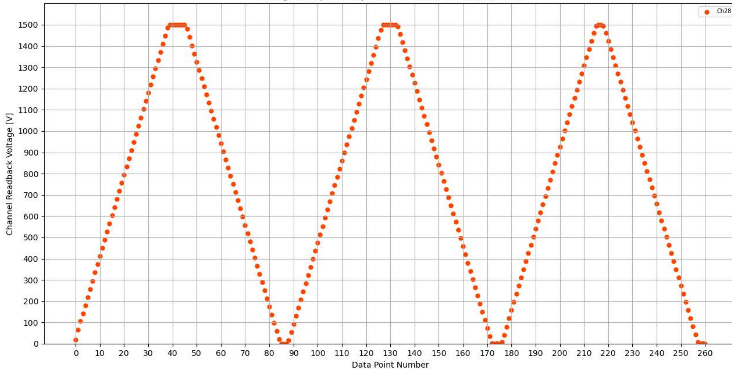
Voltage Ramp Test (Python) Bd #309, Slot #9, Ch #28
