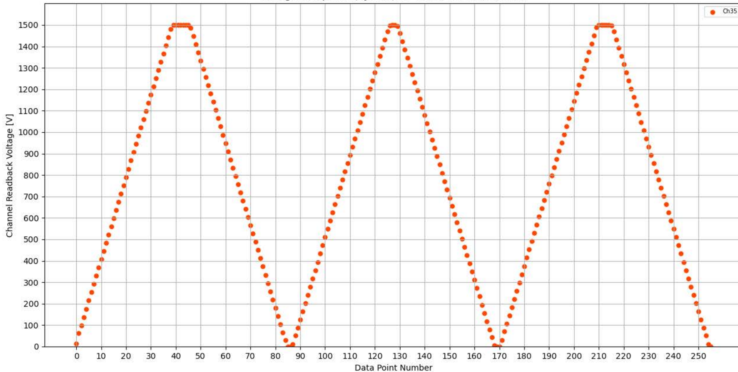
Voltage Ramp Test (Python) Bd #309, Slot #9, Ch #35
