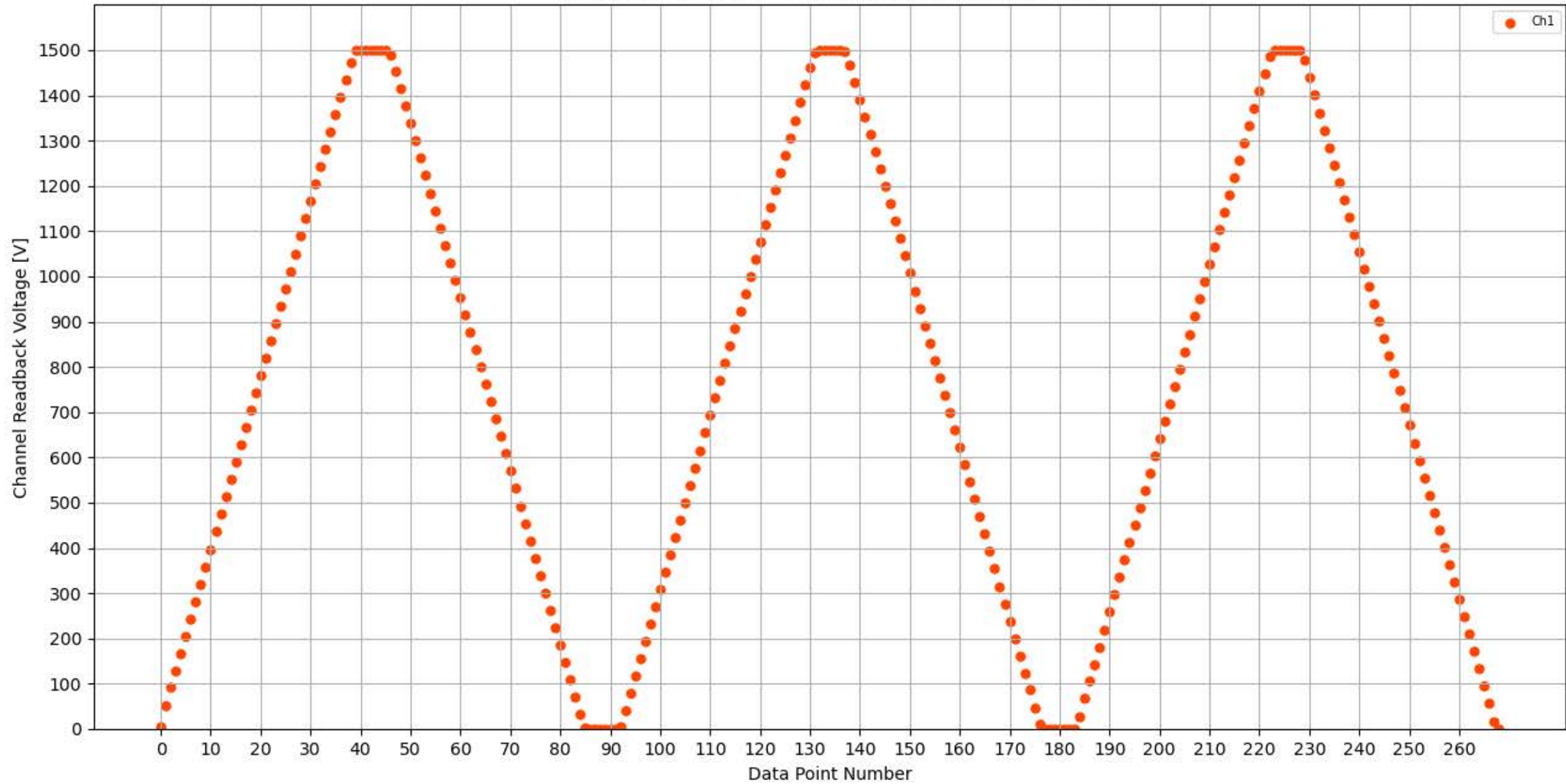
Voltage Ramp Test (Python) Bd #309, Slot #9, Ch #1
