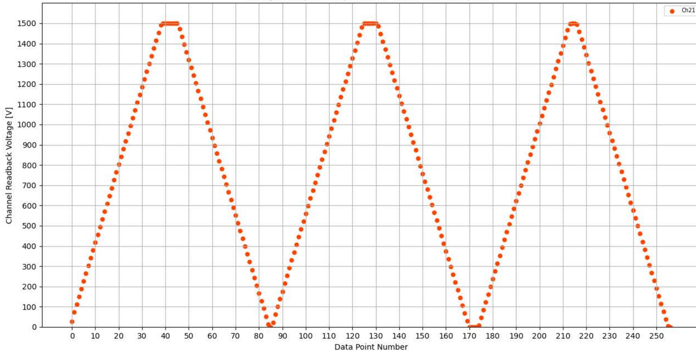
Voltage Ramp Test (Python) Bd #309, Slot #9, Ch #21
