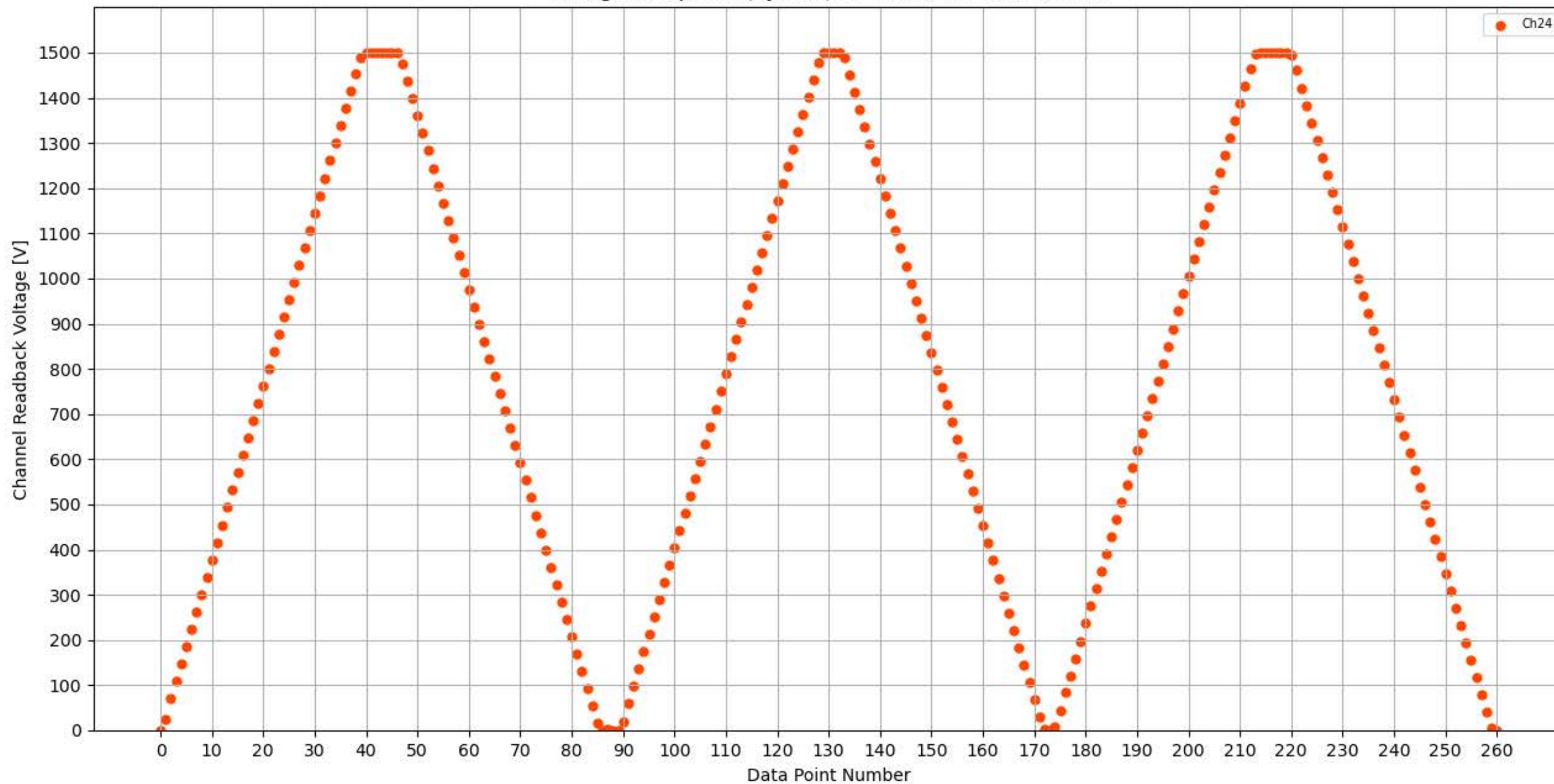
Voltage Ramp Test (Python) Bd #309, Slot #9, Ch #24
