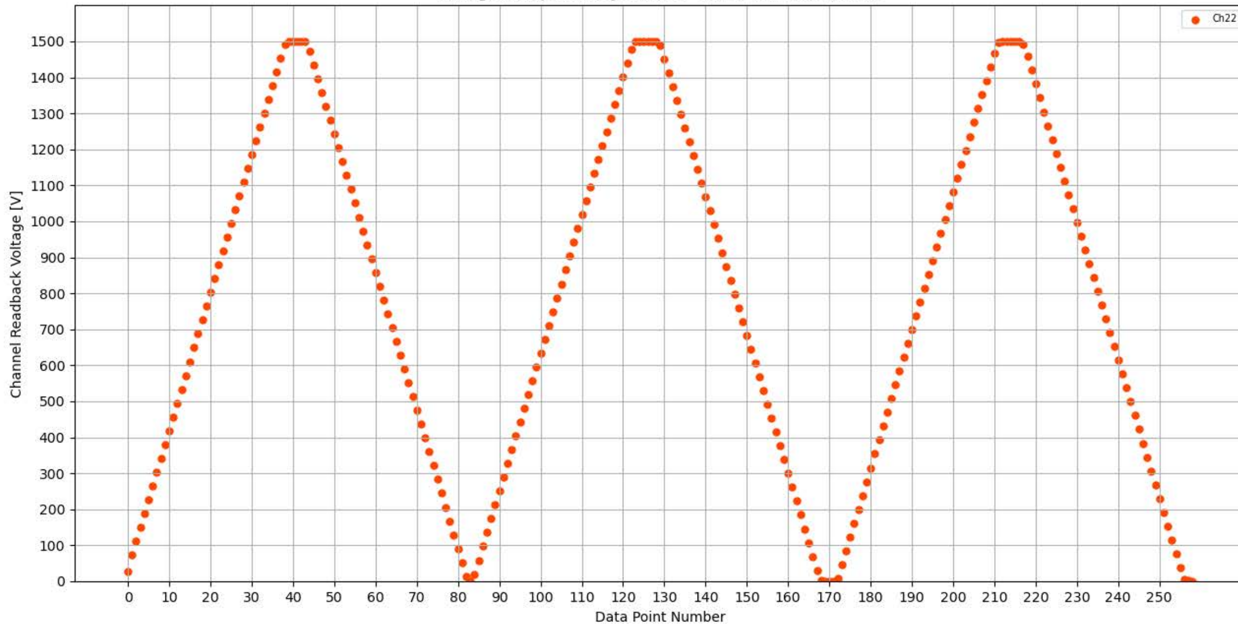
Voltage Ramp Test (Python) Bd #309, Slot #9, Ch #22
