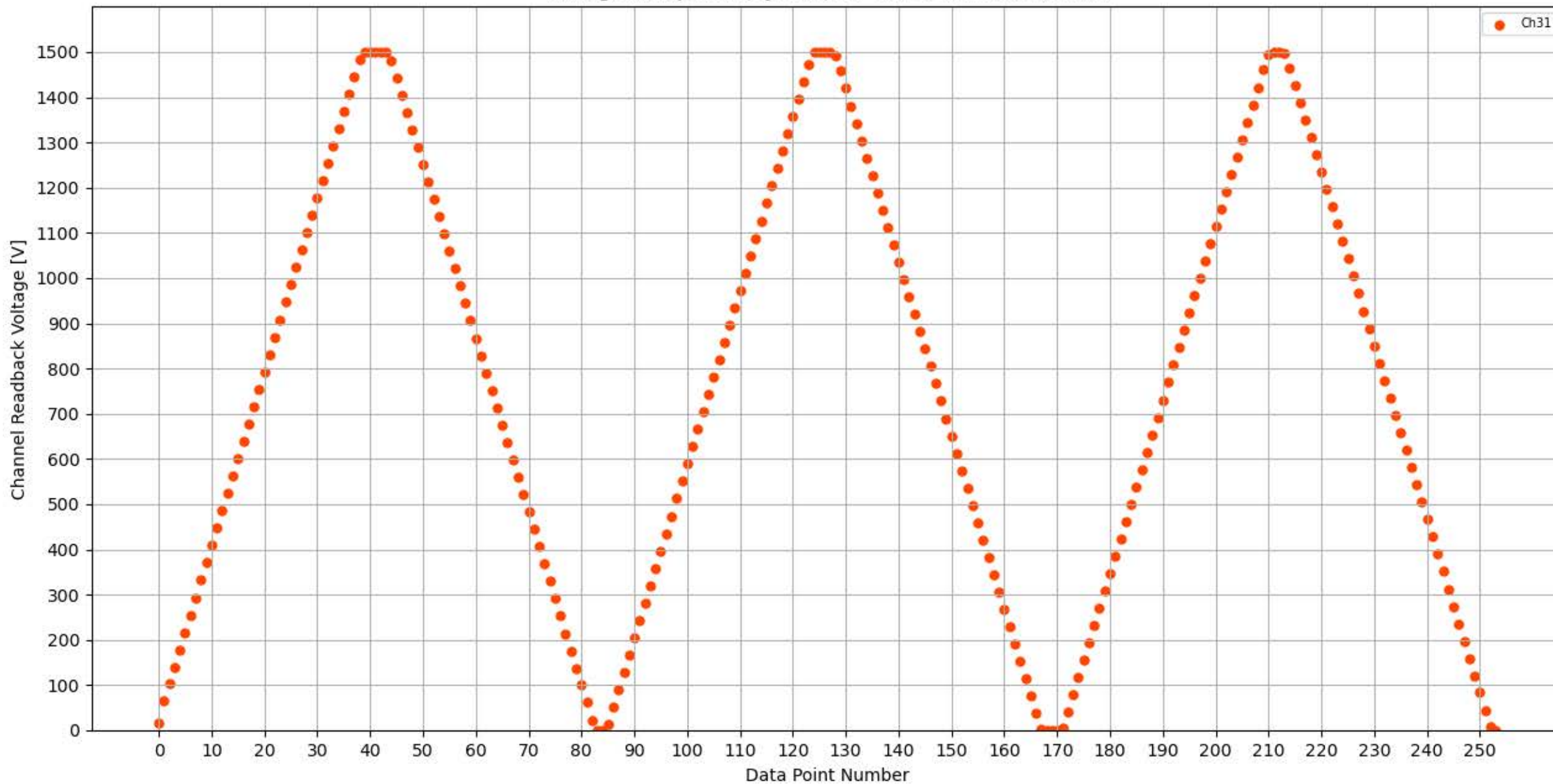
Voltage Ramp Test (Python) Bd #309, Slot #9, Ch #31
