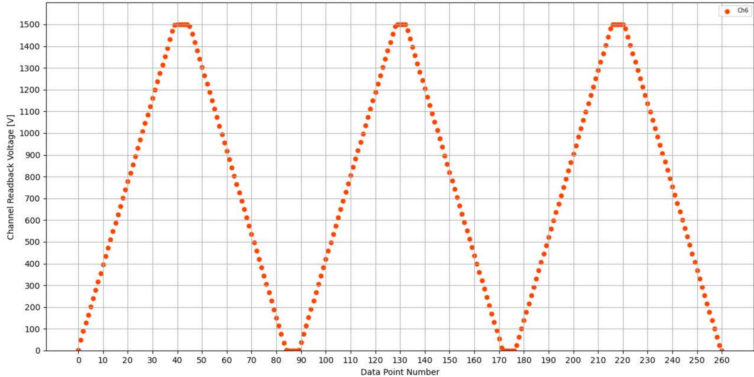
Voltage Ramp Test (Python) Bd #309, Slot #9, Ch #6
