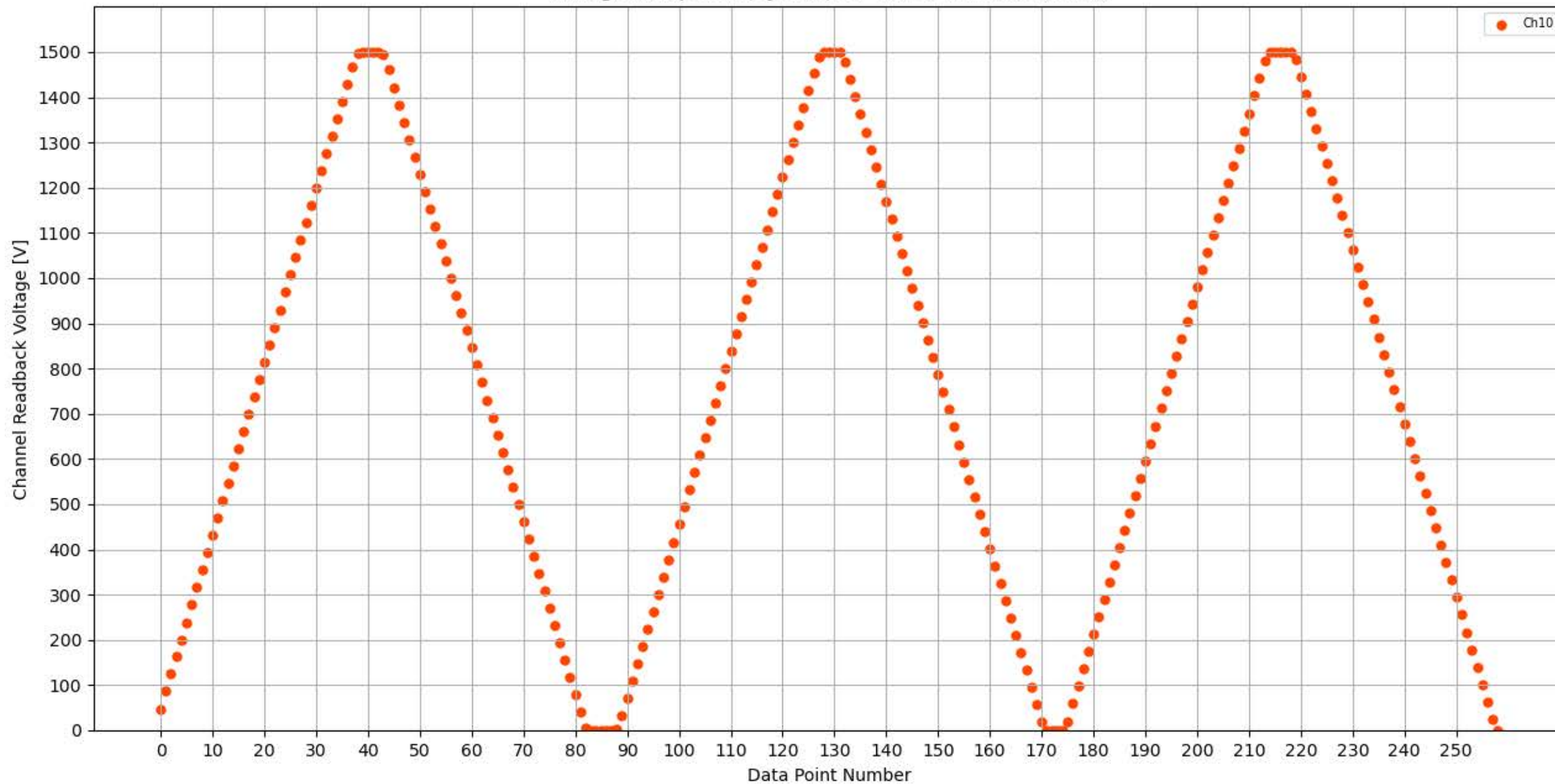
Voltage Ramp Test (Python) Bd #309, Slot #9, Ch #10
