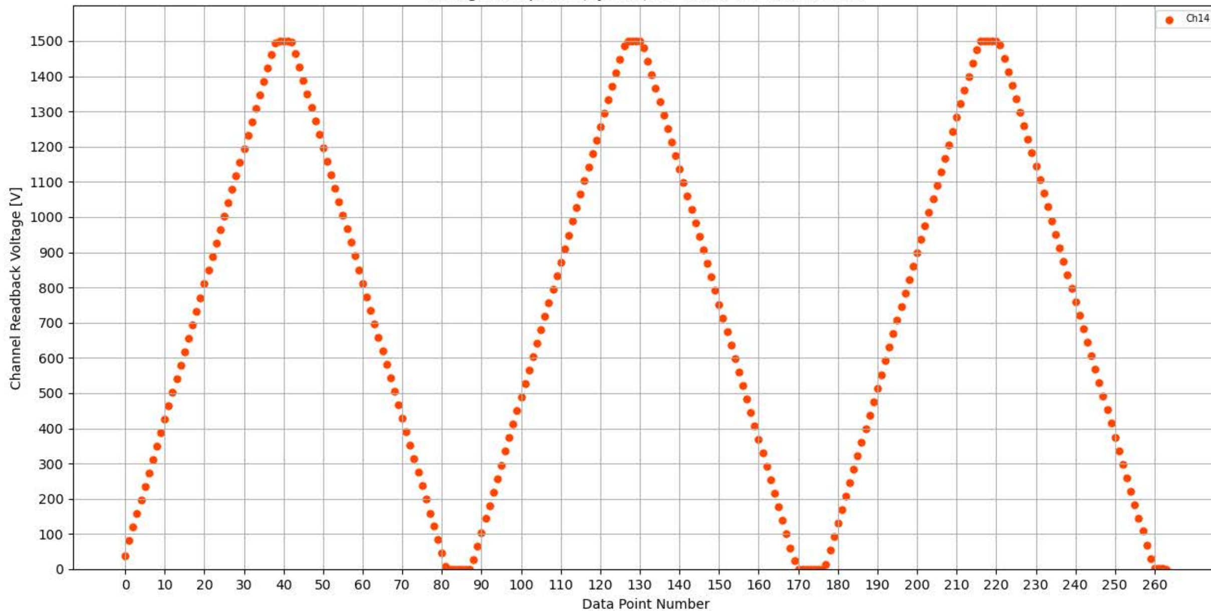
Voltage Ramp Test (Python) Bd #309, Slot #9, Ch #14
