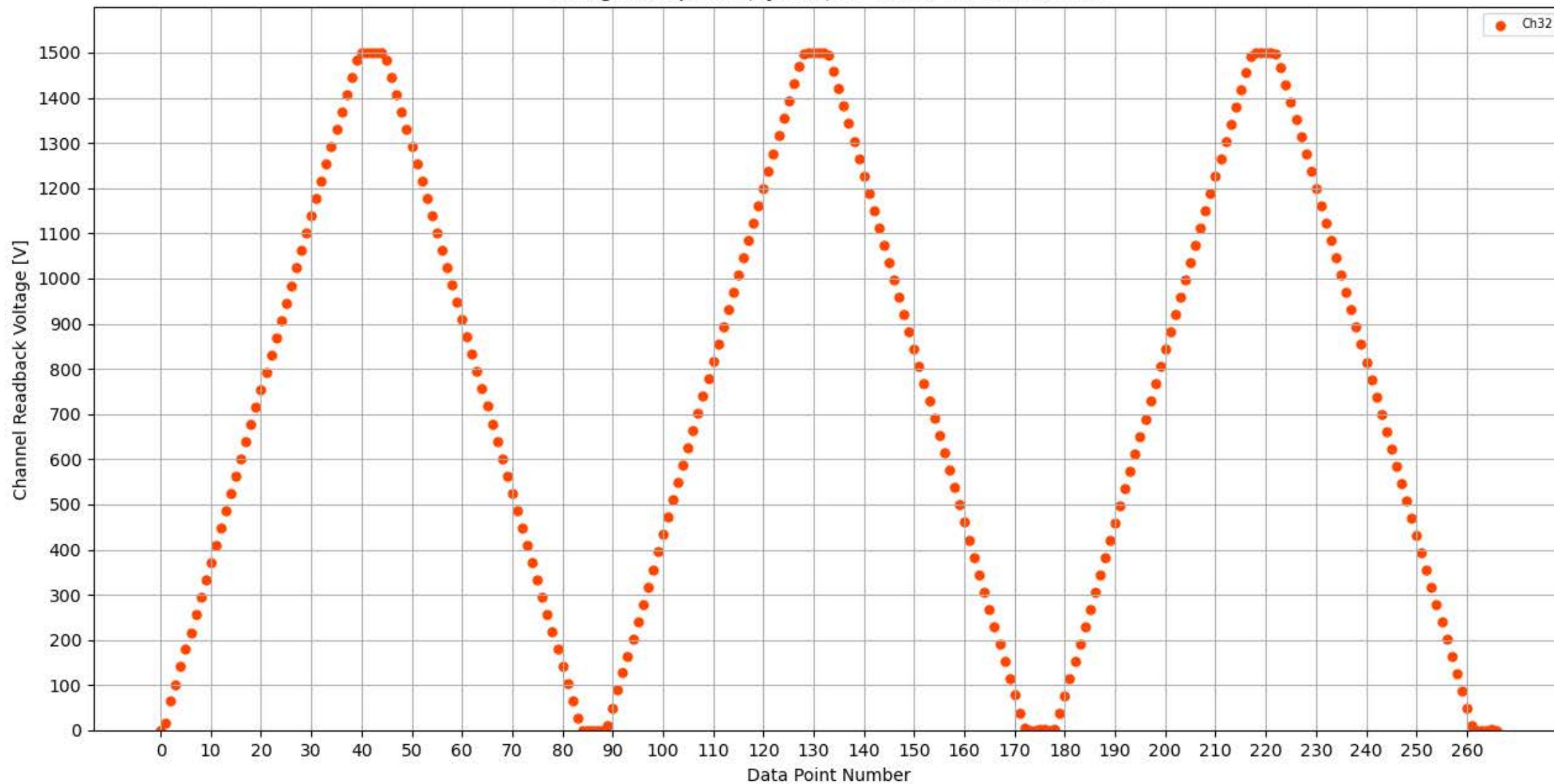
Voltage Ramp Test (Python) Bd #309, Slot #9, Ch #32
