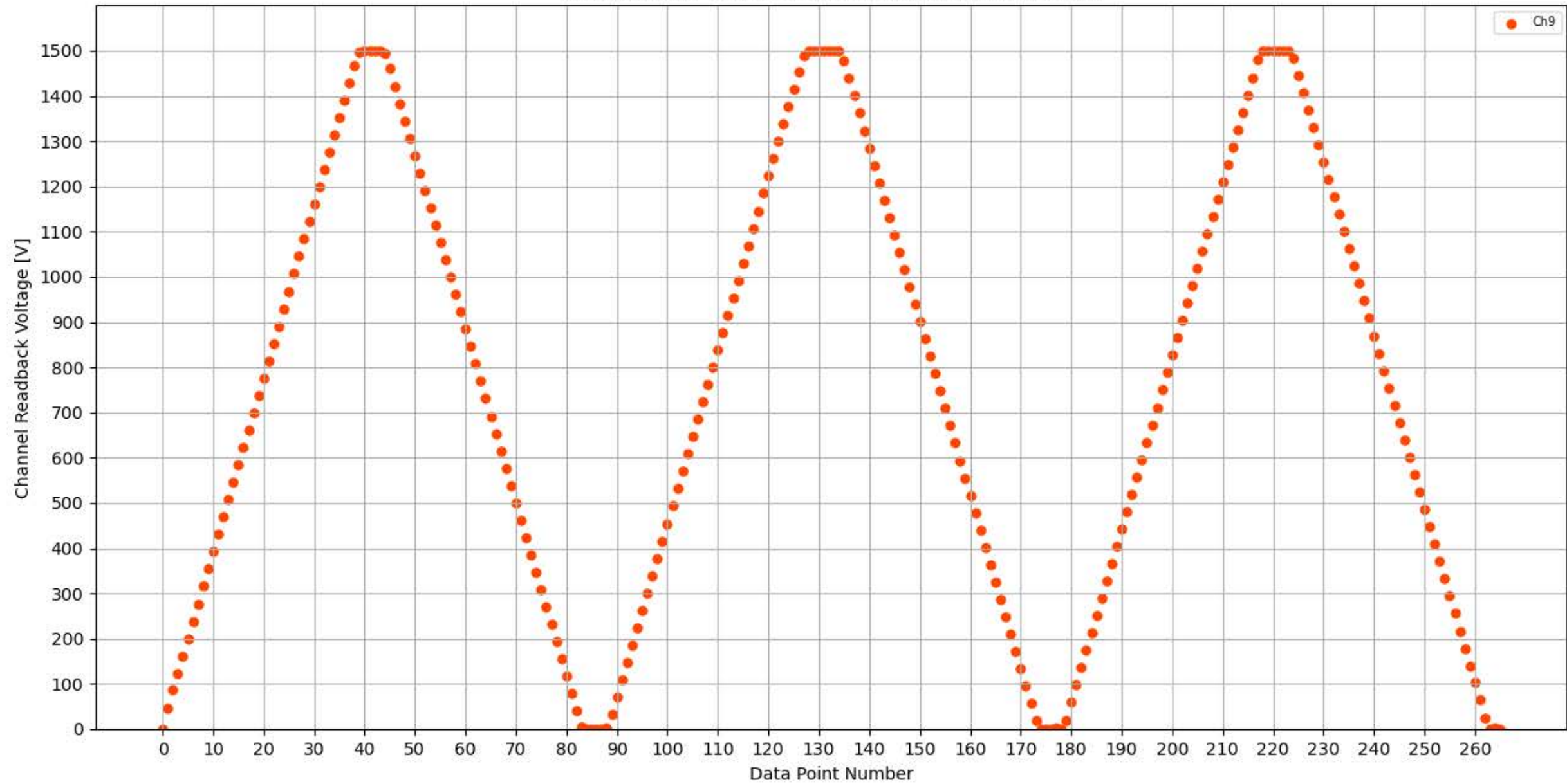
Voltage Ramp Test (Python) Bd #309, Slot #9, Ch #9
