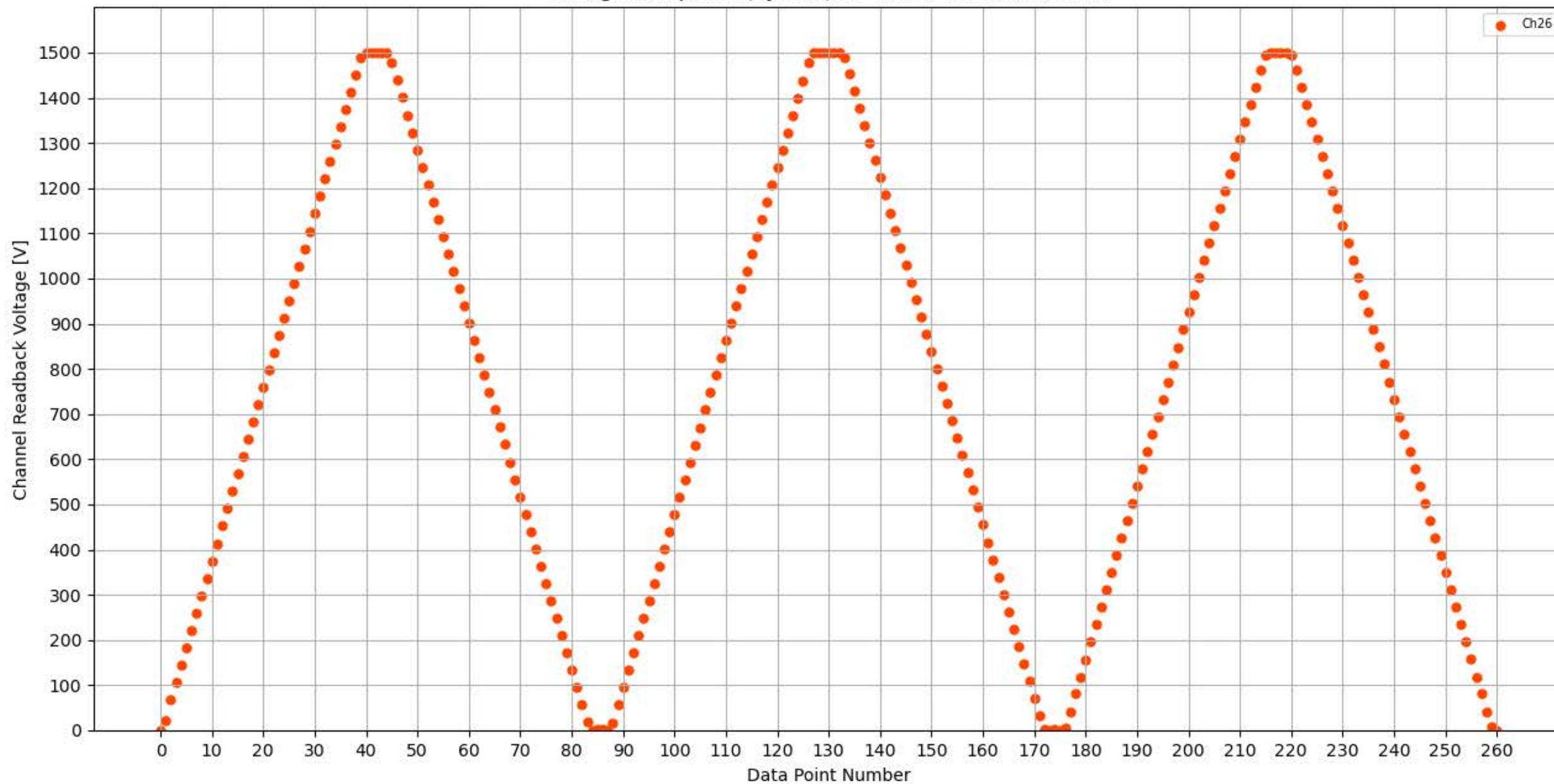
Voltage Ramp Test (Python) Bd #309, Slot #9, Ch #26
