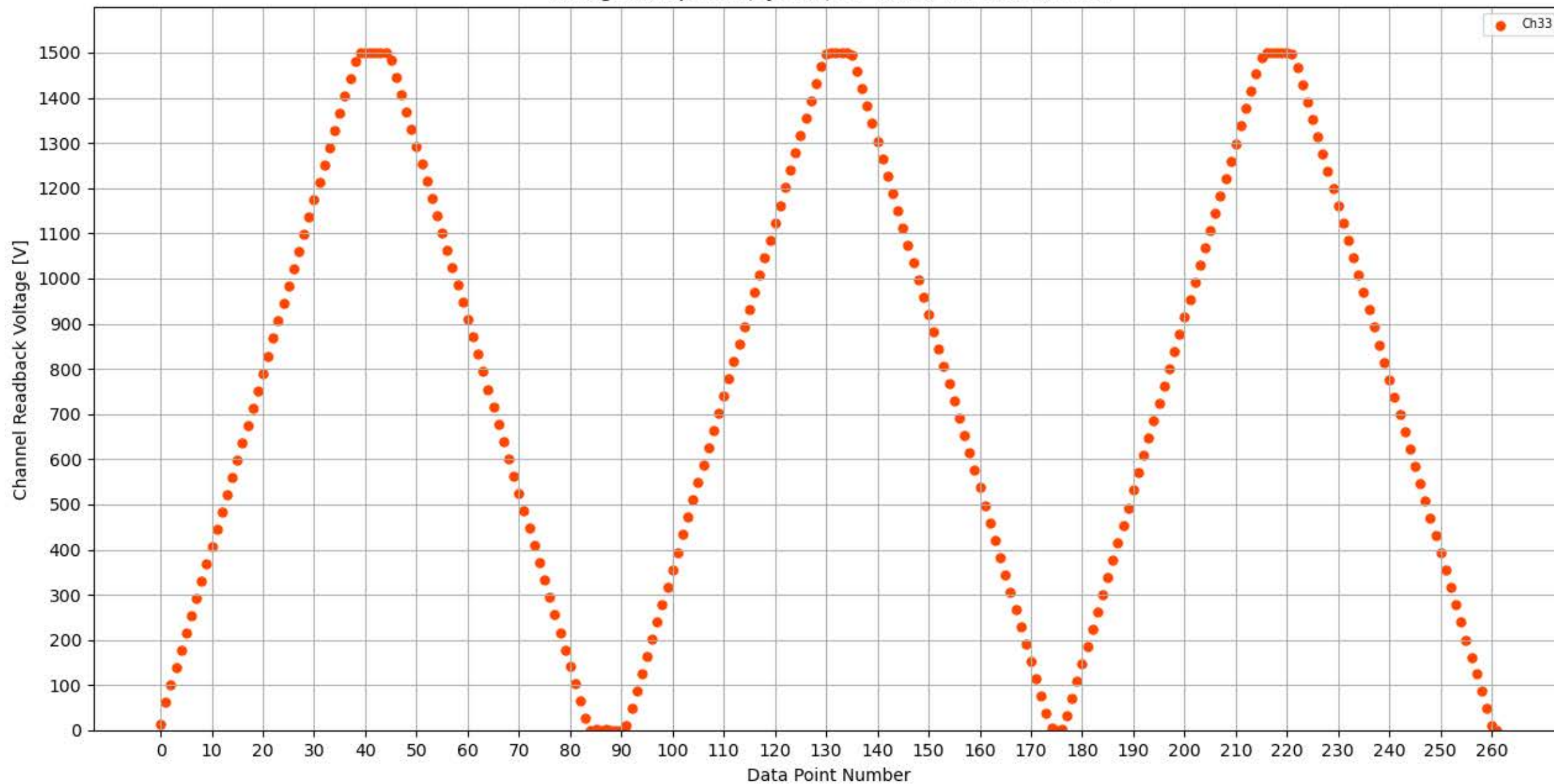
Voltage Ramp Test (Python) Bd #309, Slot #9, Ch #33
