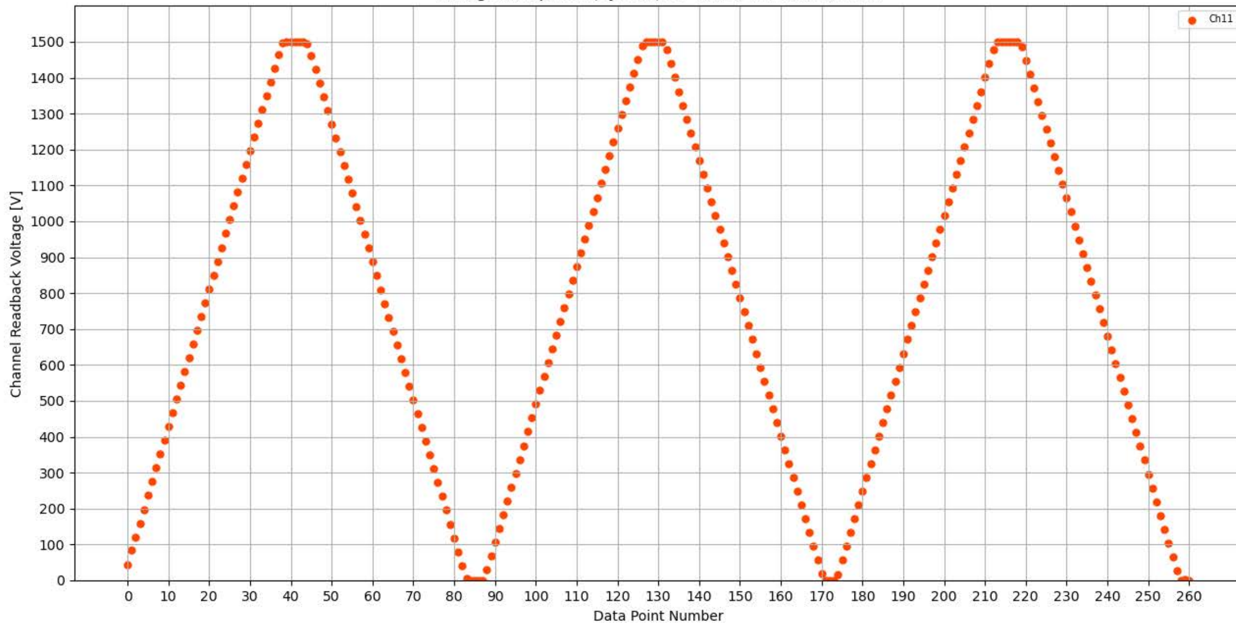
Voltage Ramp Test (Python) Bd #309, Slot #9, Ch #11
