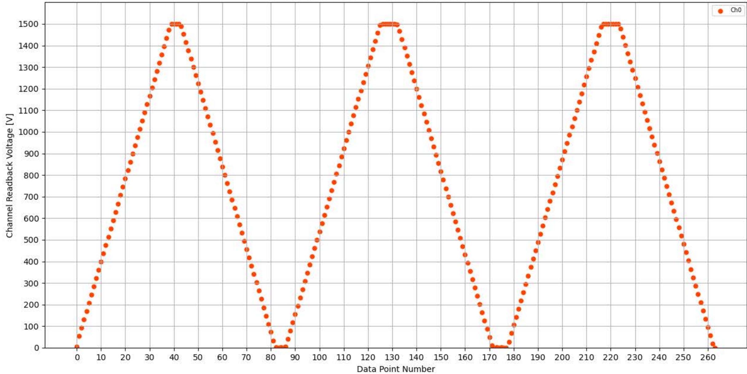
Voltage Ramp Test (Python) Bd #309, Slot #9, Ch #0
