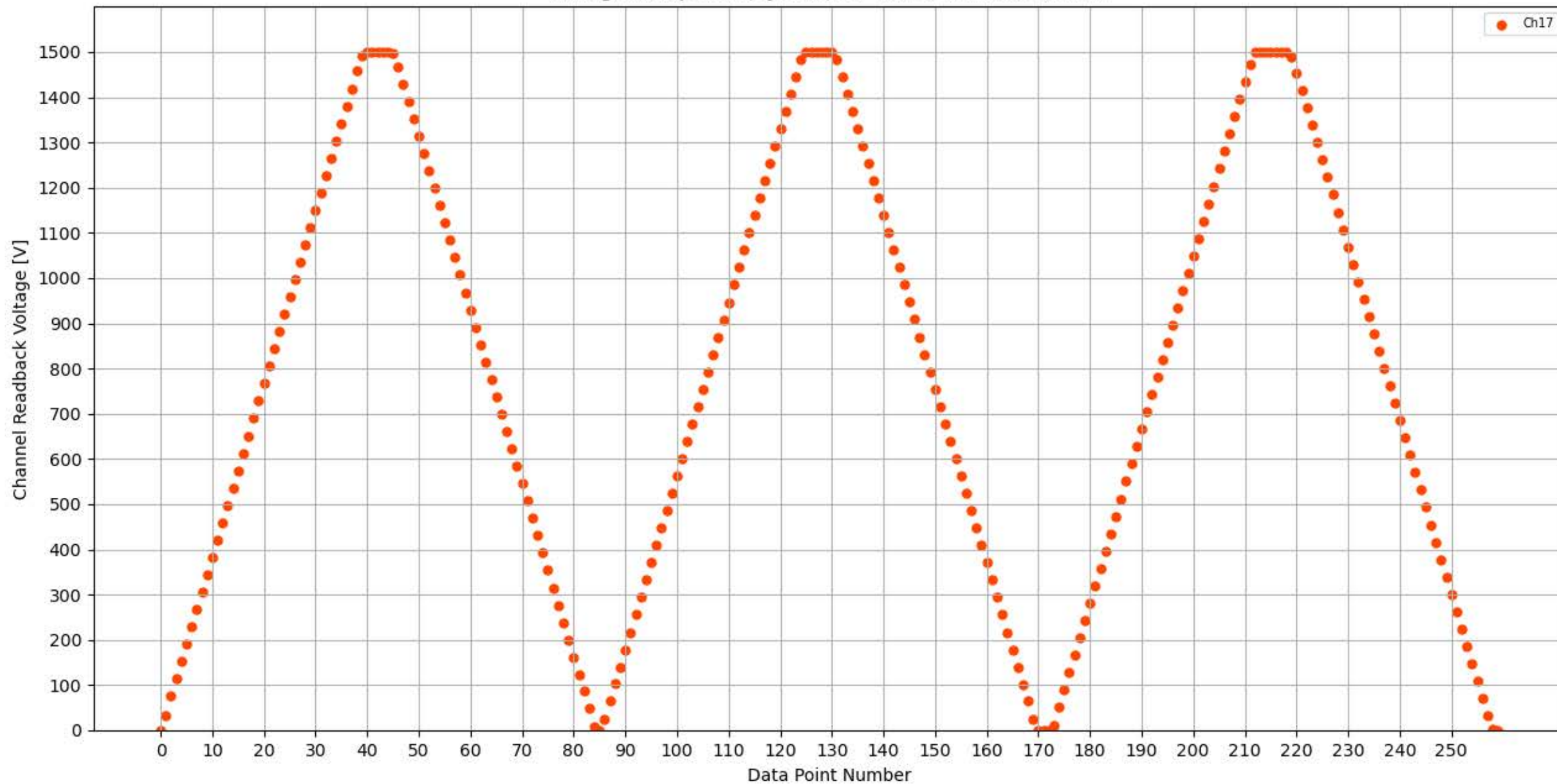
Voltage Ramp Test (Python) Bd #309, Slot #9, Ch #17
